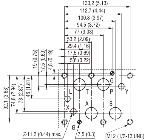
Dn 25 - ISO 4401-08-08-0-05
