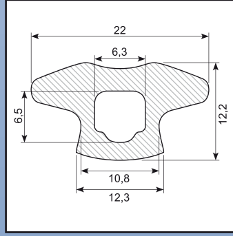
Rubber profile EPDM SH 65
