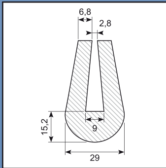
U-profile SH 70 Roll of 25 m
