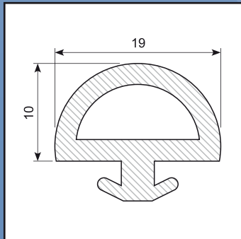
D-weatherstrip EPDM SH 60
