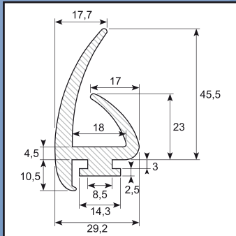
Rubber profile for alu track EPDM SH 70
