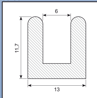
Textile / rubber Hardness: SH 70
