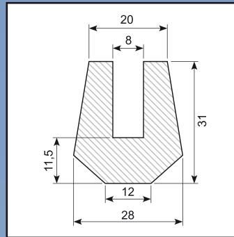
U-profile EPDM SH 70 Roll of 25 m
