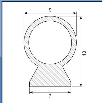
Rubber profile EPDM SH 60 / 65
