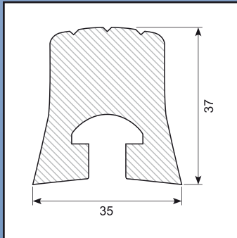
Fender profile with channel PE Length 3 m
