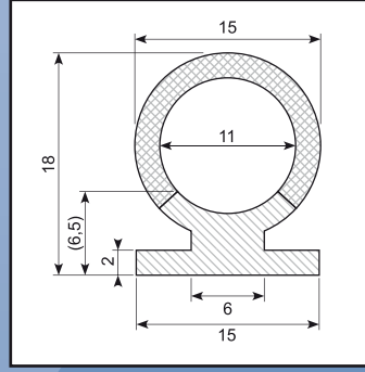
Co-ex profile EPDM / sponge rubber SH 80
