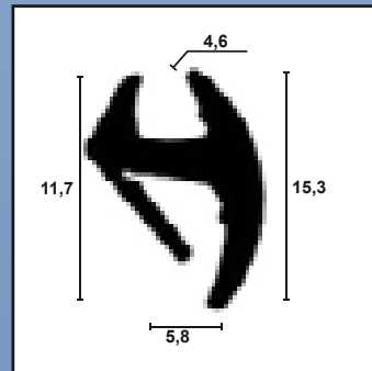
End-stop profile EPDM, Black SH 65
