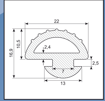
D-weatherstrip EPDM SH 70
