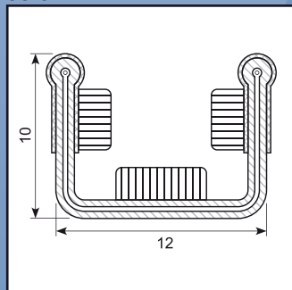
Rubber / fabric / brush 4 - 5 mm glass Steel
