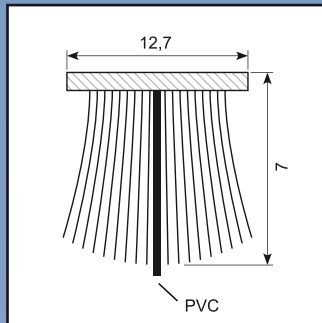
Self-adhesive list with brushes. Grey
