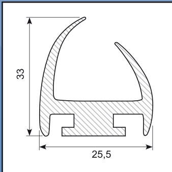
H-profile for aluminium rail EPDM SH 70
