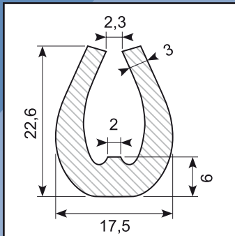
U-profile EPDM SH 80 Roll of 50 m
