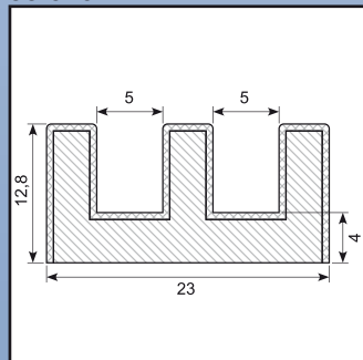
Flocked channel molding
