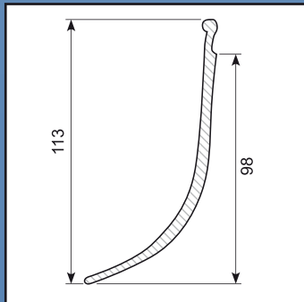
Skirt profile PVC, white Roll of 14 m
