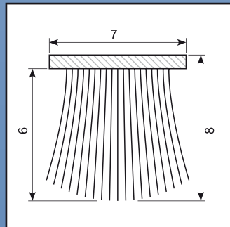
Self-adhesive list with brushes and waterproof centre film. Grey
