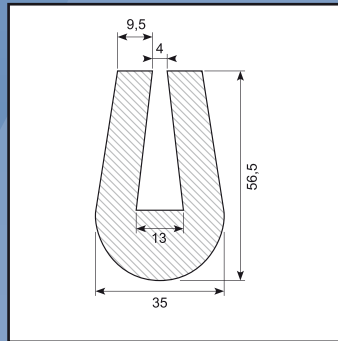
U-profile SH 65 Roll of 25 m
