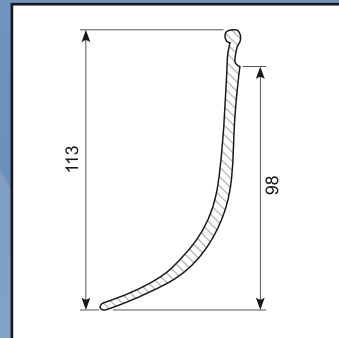
Skirt profile SH 75
