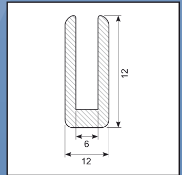
U-profile EPDM SH 70
