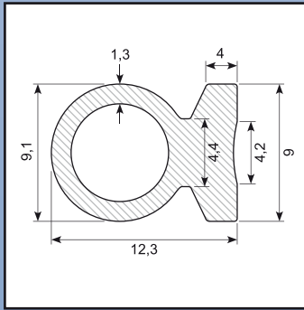
Balloon profile SH 65
