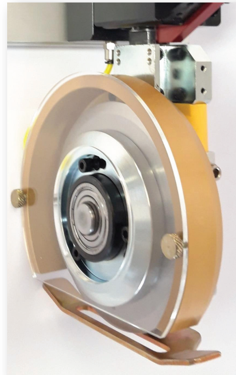
PLEXIGLASS SIDE COVER FOR BLADE
