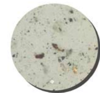
Unacceptable (ISO 21/19/17 at 100x)
