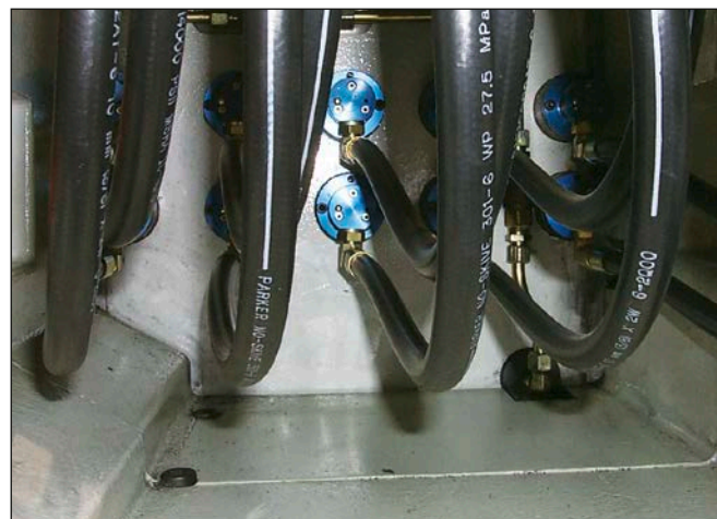
Deublin 1117 Bearingless Unions on Automotive Transfer Line.
