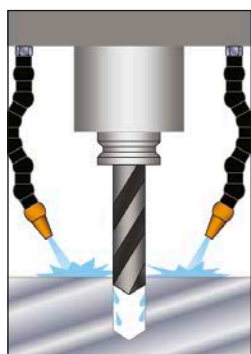
Flood Coolant
