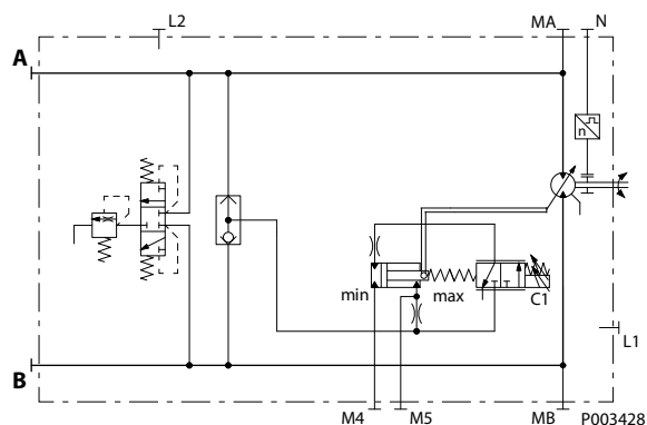
Hydraulic schematic
